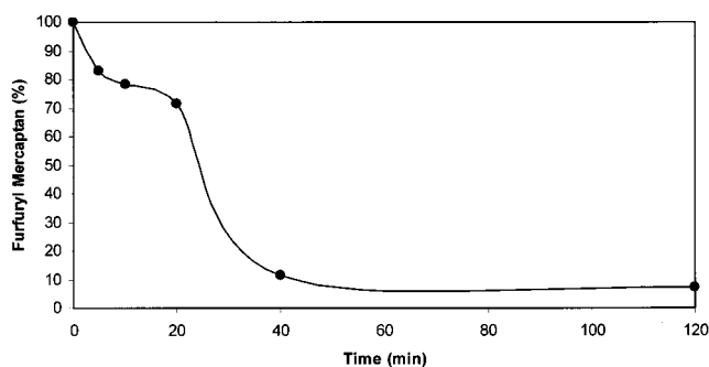
Figure 3. Degradation of furfuryl mercaptan under Fenton-type reaction conditions over a time period of 2 h.
