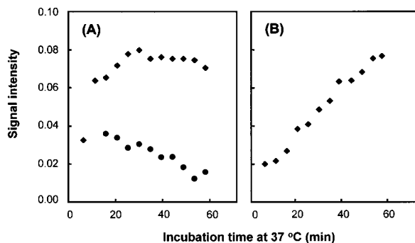
Figure 7. Variation of the intensities of the EPR signals from the \cdot\text{OH} adduct ( \blacklozenge ), along with that of the unidentified adduct with high- and low-field peaks separated by 12.2 mT ( \bullet ), as a function of incubation time with DEPMPO at 37^\circ\text{C} of (A) sample 5, which contained no ascorbic acid, and (B) sample 5, but without furfuryl mercaptan.
