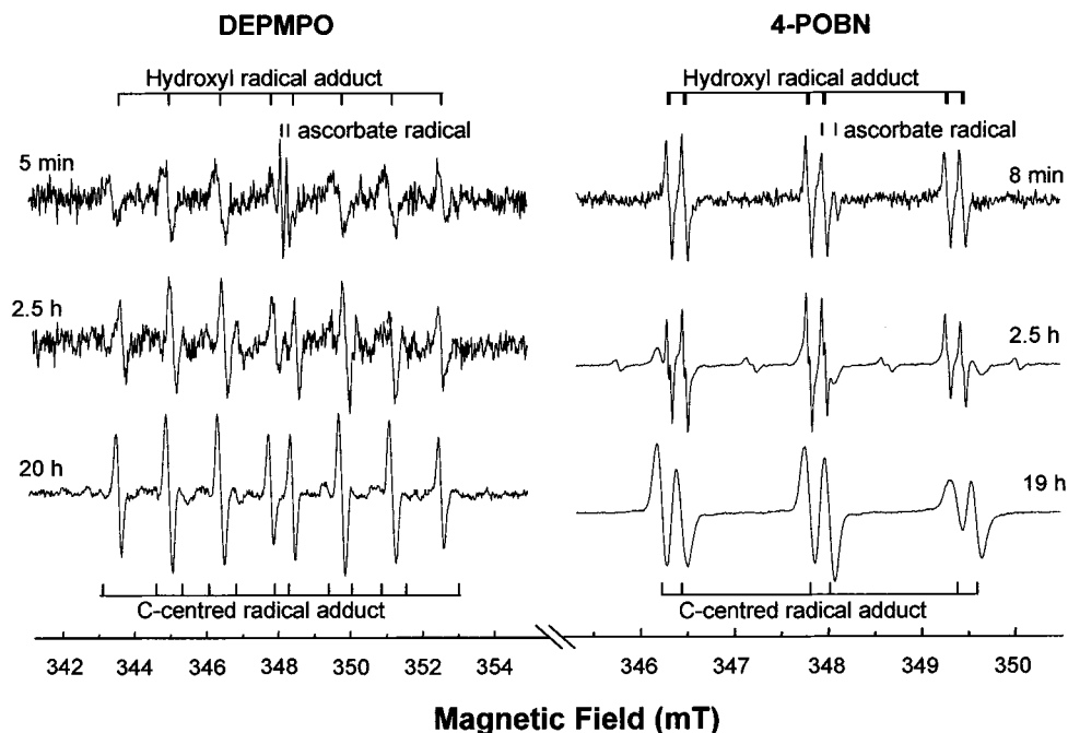
Figure 5. Representative EPR spectra obtained during incubation of model solution 1 with the spin trap DEPMPO or 4-POBN at room temperature ( \sim 20^\circ\text{C} ).
