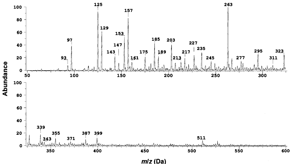
Figure 2. ESI-MS of a sample containing furfuryl mercaptan, hydrogen peroxide, and \text{FeCl}_3 in the molar ratio of 10:1:1.
