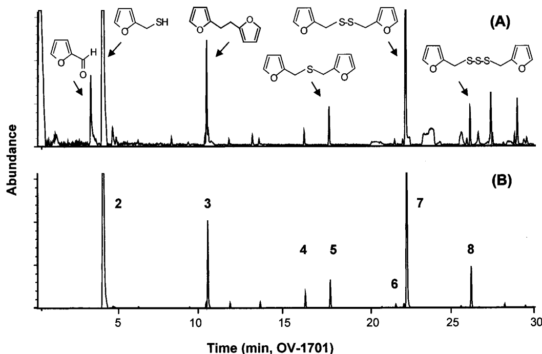
Figure 1. GC-MS identification of volatile compounds detected in a sample containing furfuryl mercaptan, hydrogen peroxide, and iron(III) ions in the molar ratio of 10:1:1: (A) total ion current; (B) extract thereof showing only the trace of m/z 81. Numbering corresponds to that in Table 5.
