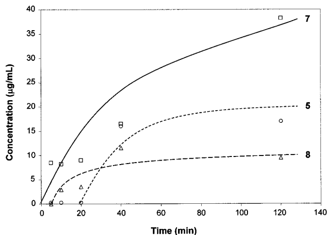
Figure 4. General tendency in the formation of difurfuryl monosulfide (○, 5 ), difurfuryl disulfide (□, 7 ), and difurfuryl trisulfide (△, 8 ) over time as degradation products of furfuryl mercaptan under Fenton conditions.
