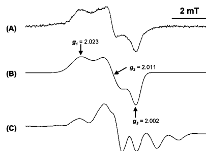
Figure 8. (A) EPR spectrum at 77 K from a rapidly frozen solution of furfuryl mercaptan in a simple model Fenton reaction system; (B) a simulation of spectrum (A) with g values of 2.002, 2.011, and 2.023 and a Gaussian line shape; (C) spectrum obtained at 77 K from furfuryl mercaptan that had received 100 Gy of \gamma -radiation from a ^{137}\text{Cs} source.
