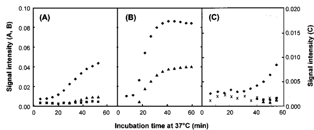
Figure 6. Variation of the intensities of the EPR signals from \cdot\text{OH} ( \blacklozenge ) and C-centered radical ( \blacksquare ) adducts along with those of the unidentified adduct with high- and low-field peaks separated by 11.6 mT ( \blacktriangle ) and 10.4 mT ( \times ) as a function of incubation time with DEPMPO at 37^\circ\text{C} of (A) sample 1, (B) sample 1 minus furfuryl mercaptan, and (C) sample 4, which contained no EDTA.
