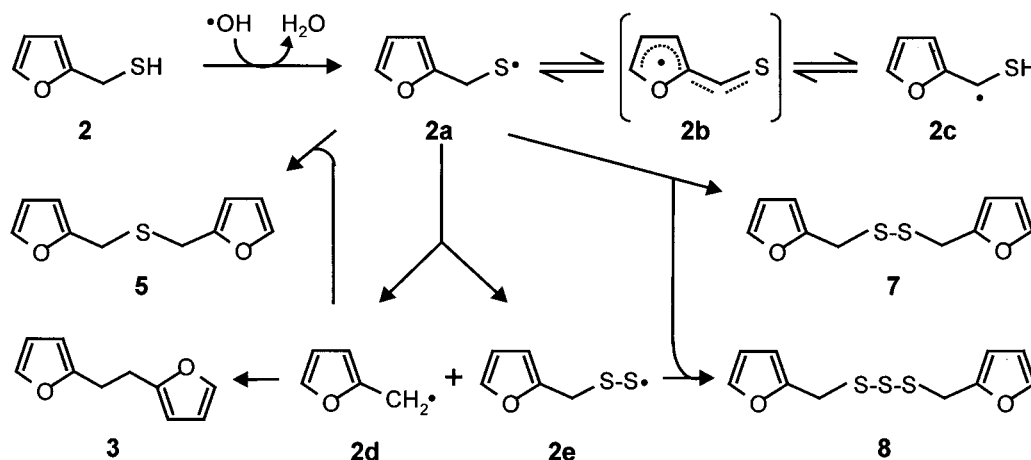
Figure 9. Hypothetical mechanism showing the degradation of furfuryl mercaptan ( 2 ) under Fenton conditions and the formation of volatile reaction products identified in this study, that is, bifurfuryl ( 3 ), difurfuryl monosulfide ( 5 ), difurfuryl disulfide ( 7 ), and difurfuryl trisulfide ( 8 ).
